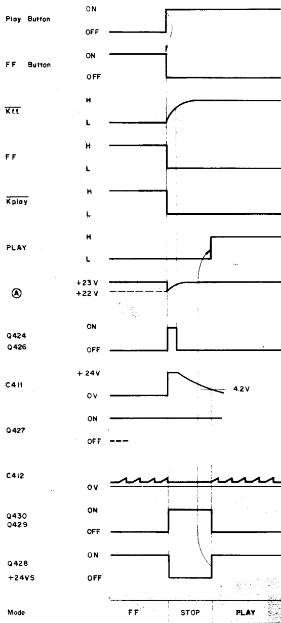
Fig. 2.3.7 Timing Chart
