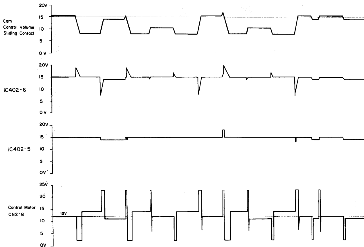
Fig. 2.3.11 Timing Chart
