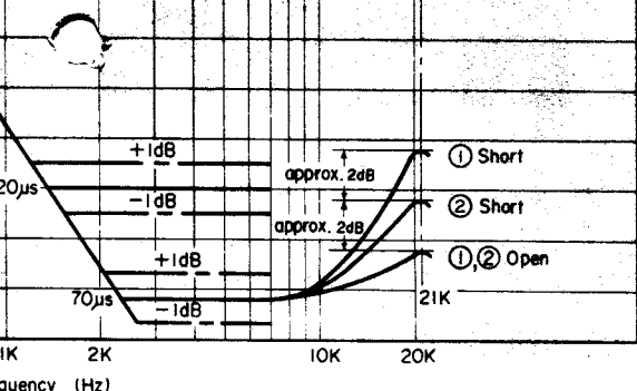
Equalization Curve
