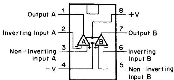
Fig. 14.2 Operational Amp. IC 4558
