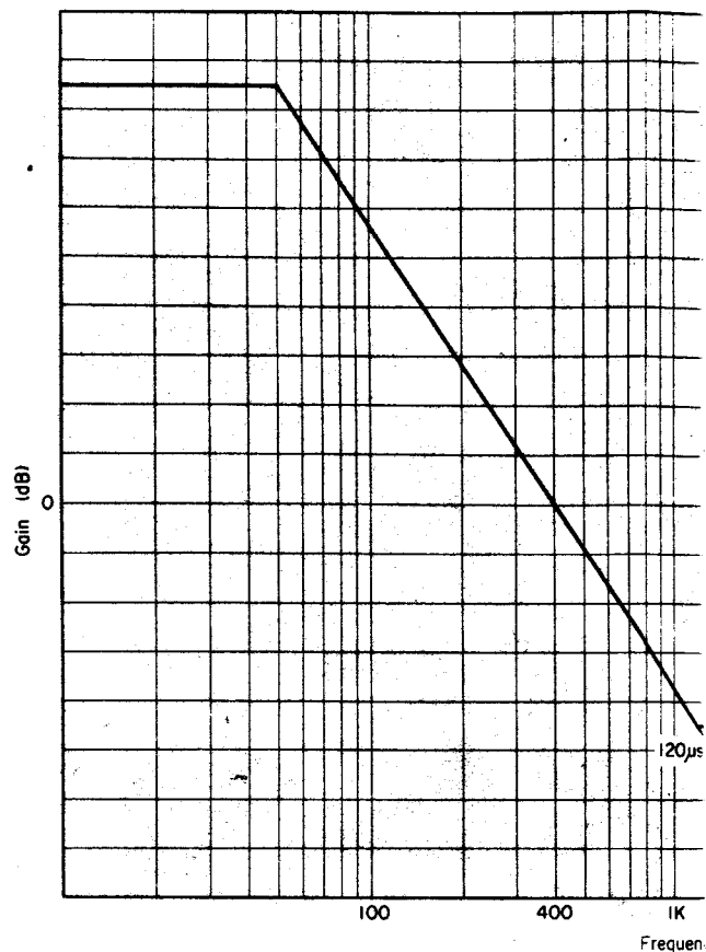
Fig. 7.7 Playback Eq.
