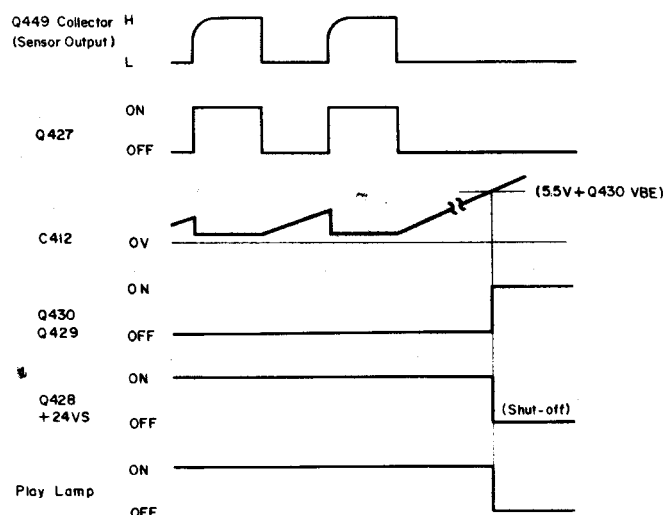
Fig. 2.3.6 Timing Chart
