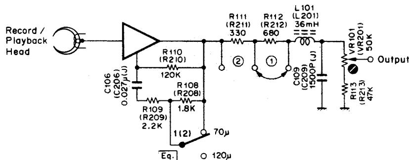
Fig. 7.8 Playback Amp.
